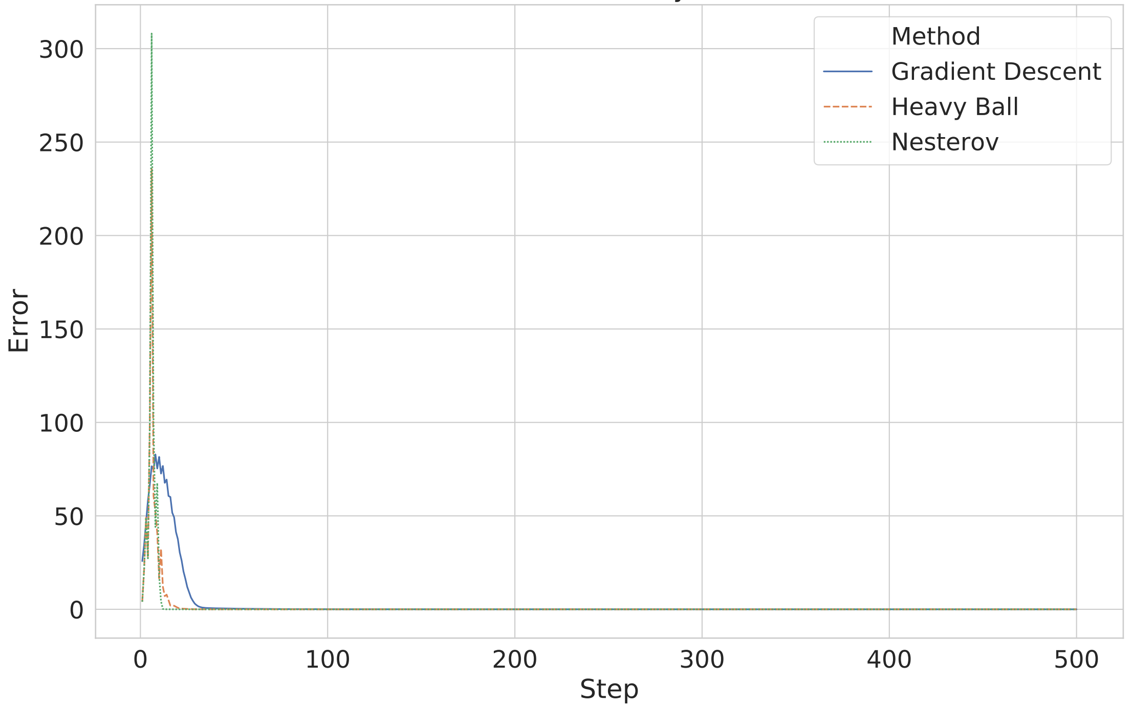
Error ratios for GD vs Heavyball vs Nesterov
