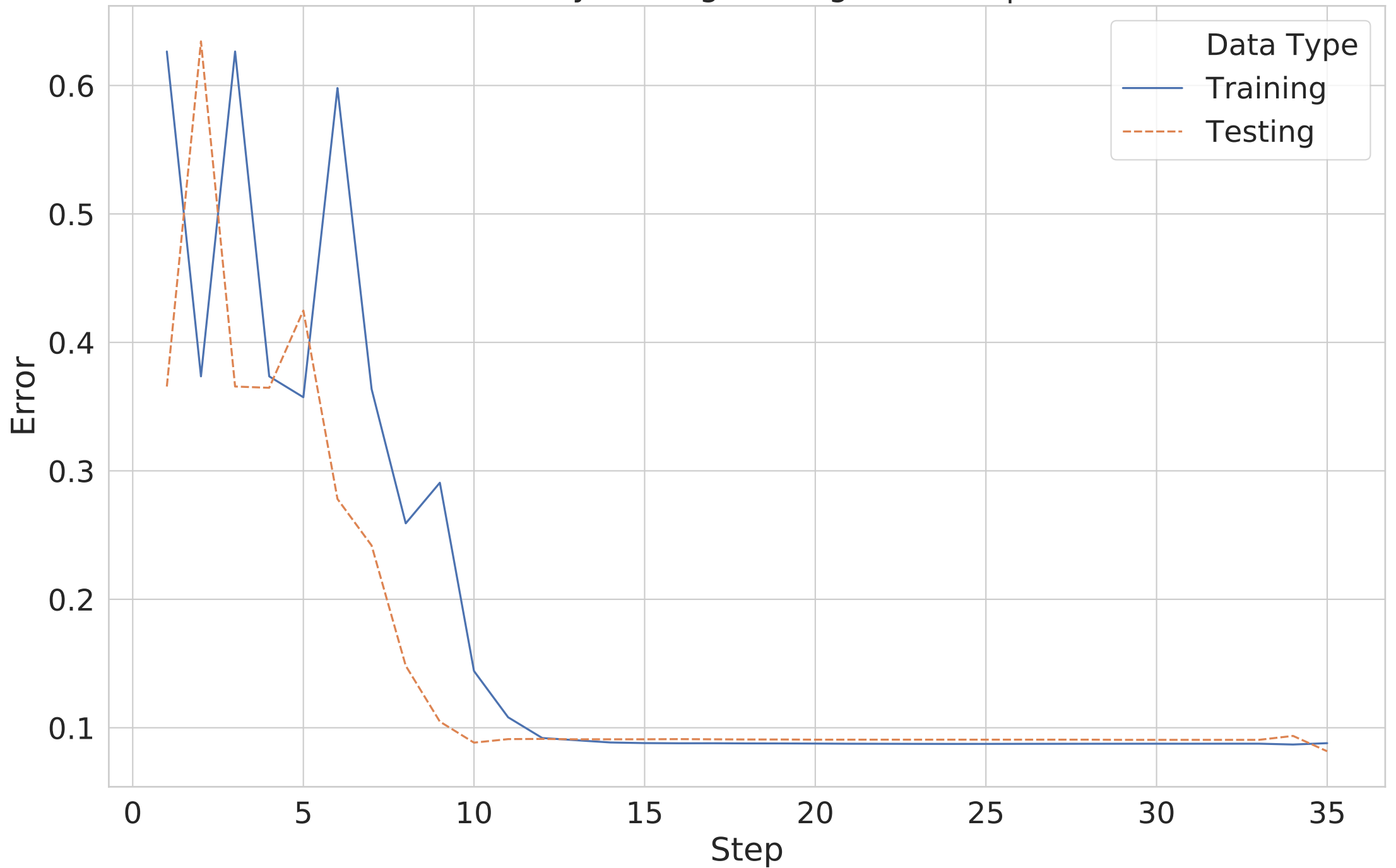
Error [0-1] for heavy ball logistic reg. ( \eta=1 ) | Problem 3(e)
