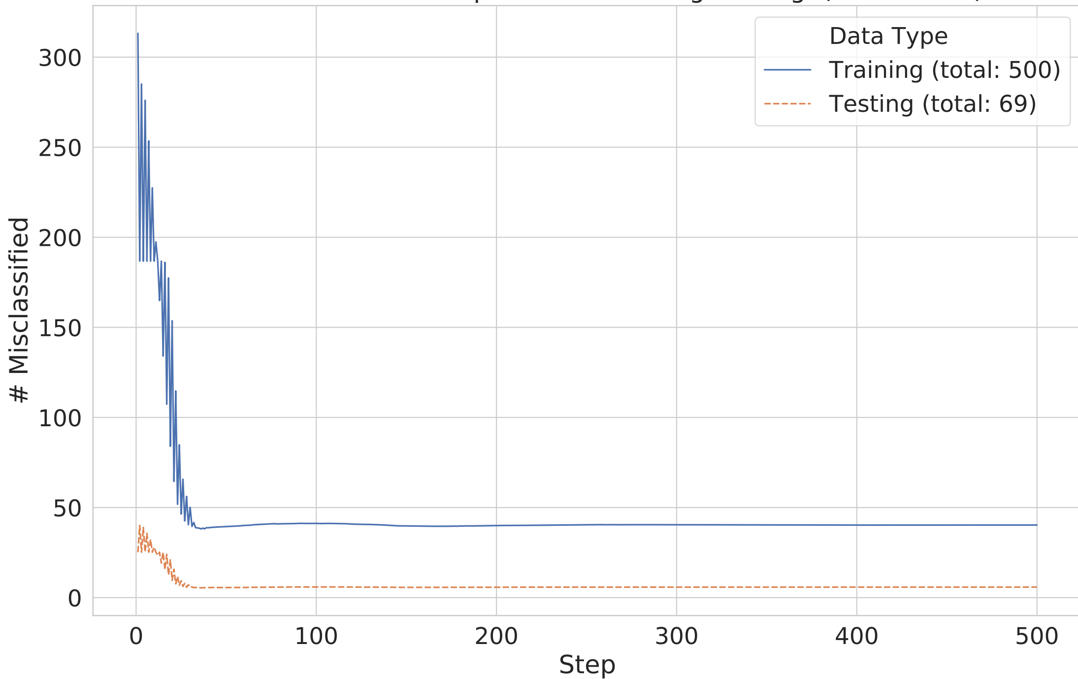
# of Misclassified samples for vanilla logistic reg. (Problem 3c)
