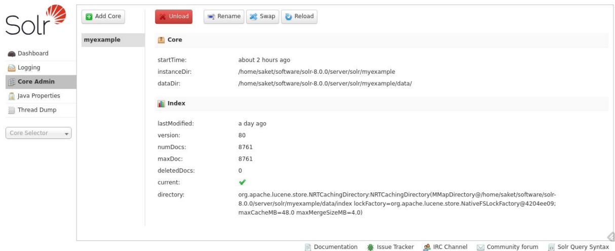
Figure 2. Core admin page for 'myexample'.
