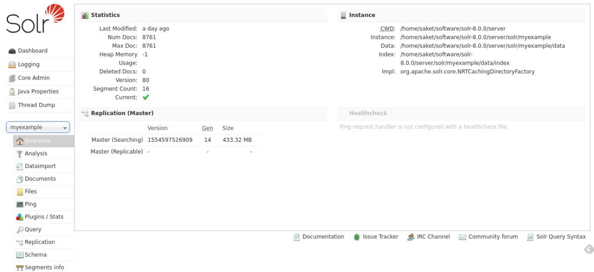
Figure 1. Solr page running on http://nucleus.usc.edu:8983/solr/#/myexample/core-overview
